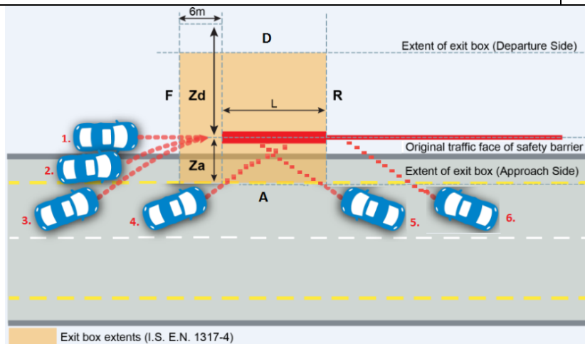
Exit box extents (I.S. E.N. 1317-4)
